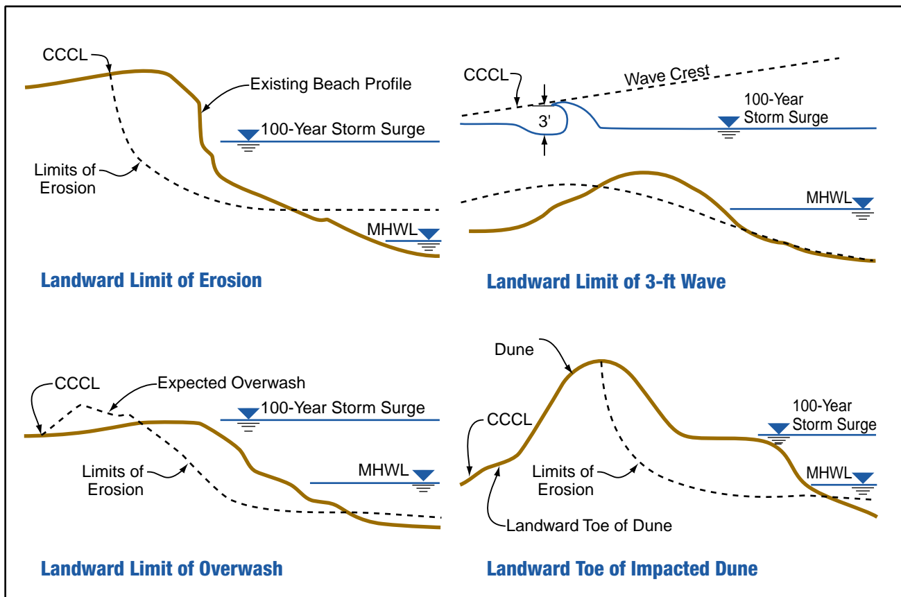
Figure G-7 Criteria used to establish Florida's Coastal Construction Control Line (CCCL) (from Olsen 1987).
