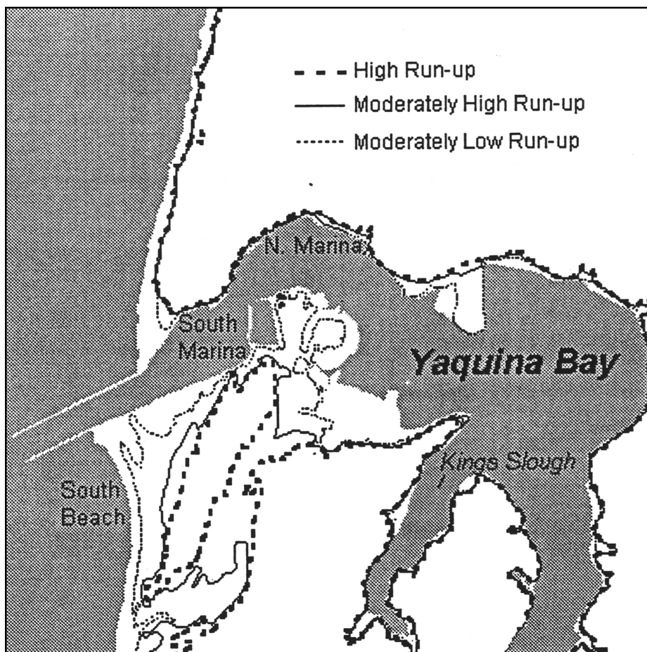
Figure G-20 Yaquina Bay, Oregon, tsunami inundation map (from Priest et al. 1997).
