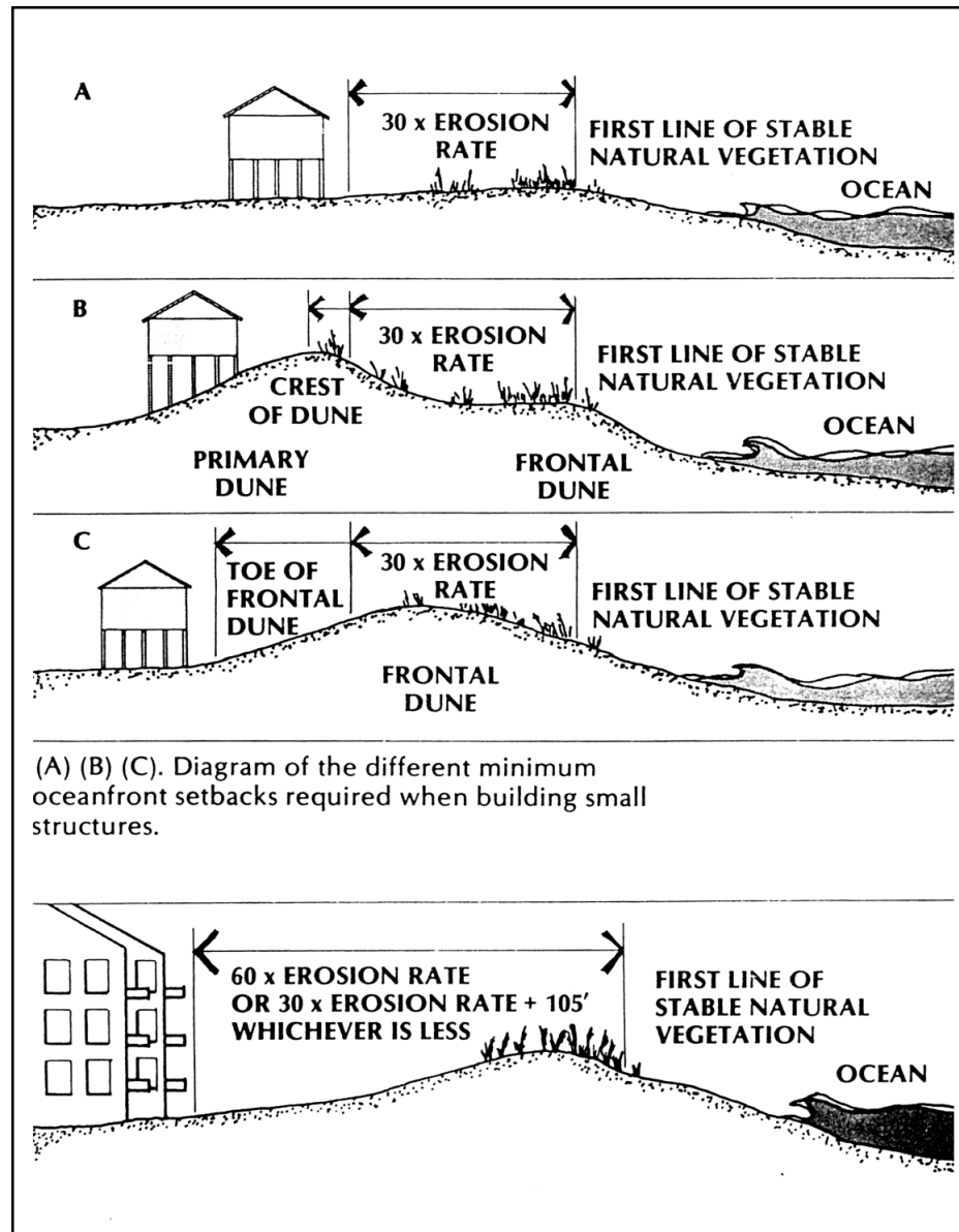
Figure G-9 Minimum setbacks in North Carolina Ocean Erodible Areas.
