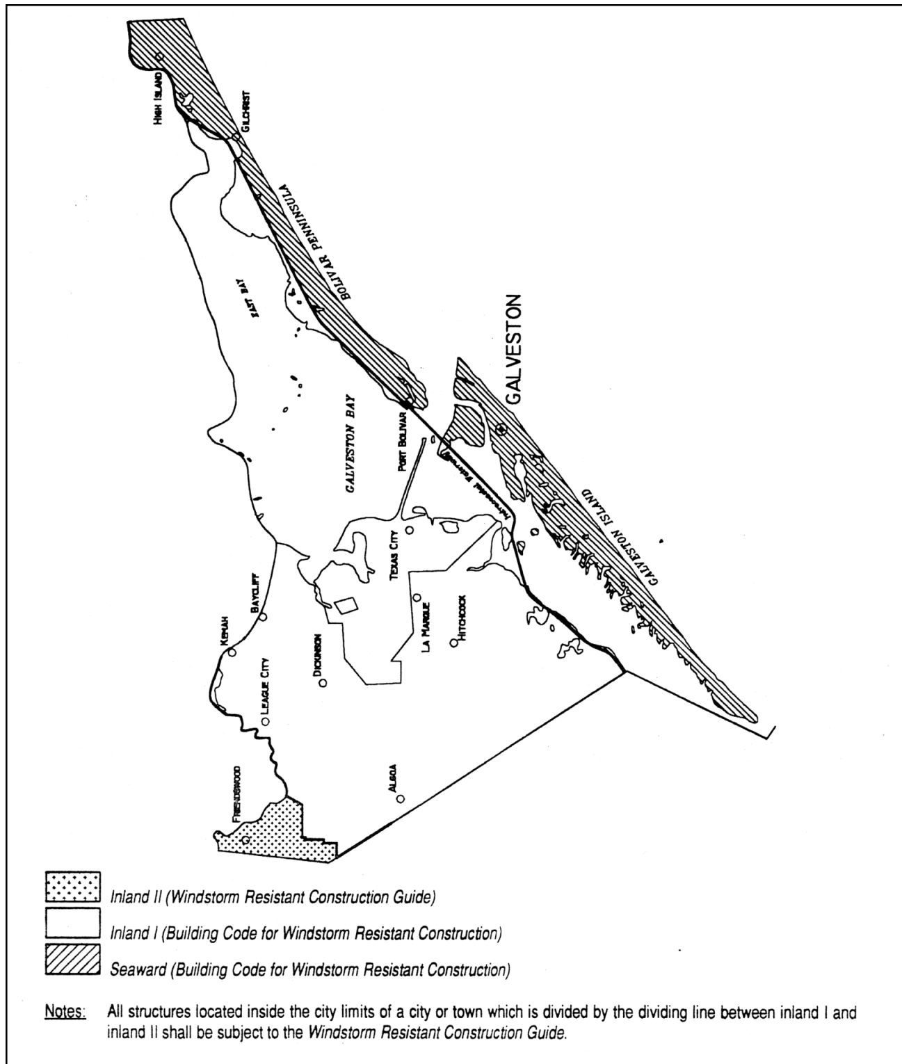
Figure G-26 Texas Department of Insurance construction zones, Galveston County, Texas (from Texas Department of Insurance 1998).
