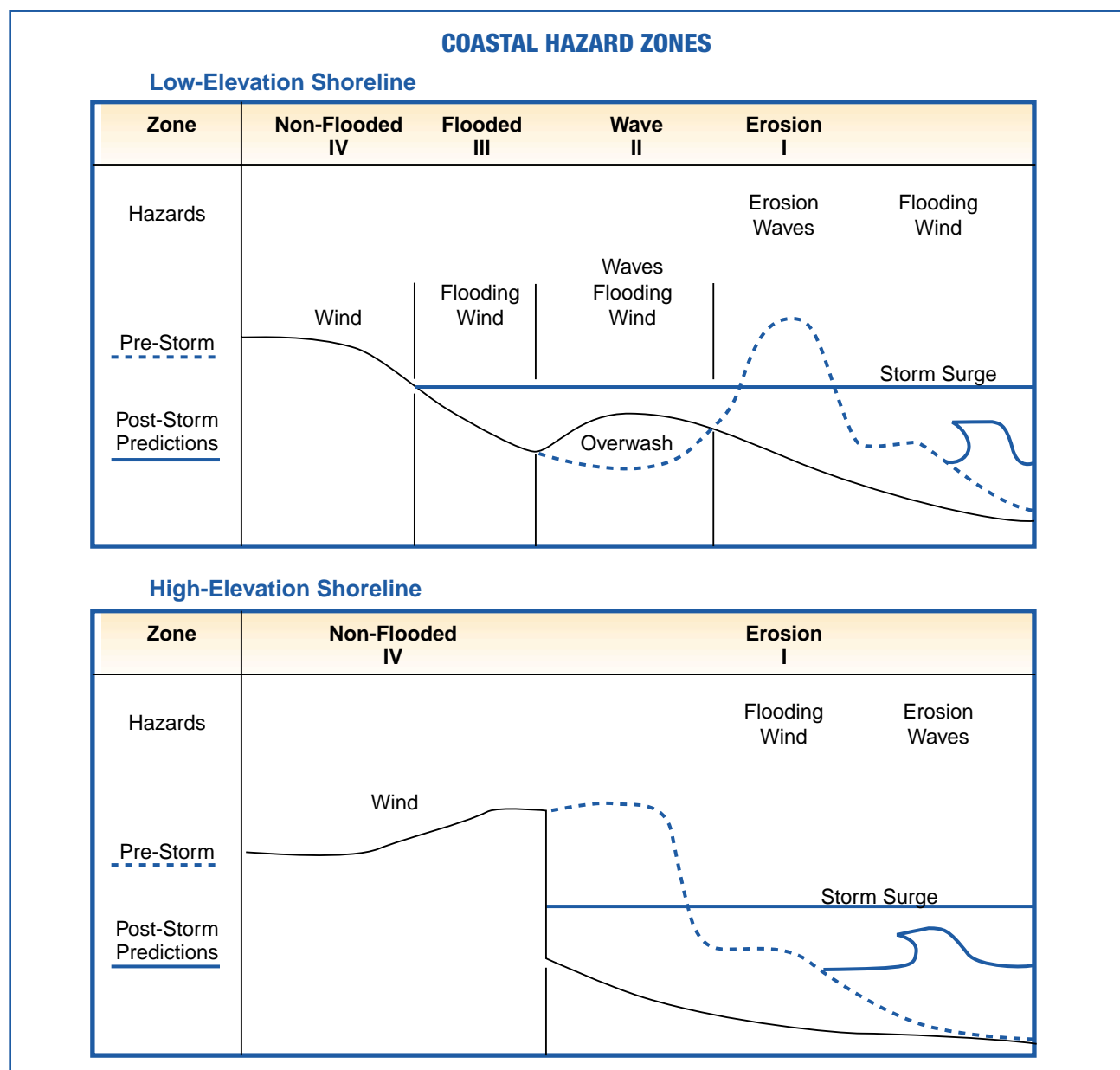
Figure G-4 Coastal hazard zones for low-elevation and high-elevation shorelines in Texas (from Rogers 1990).
