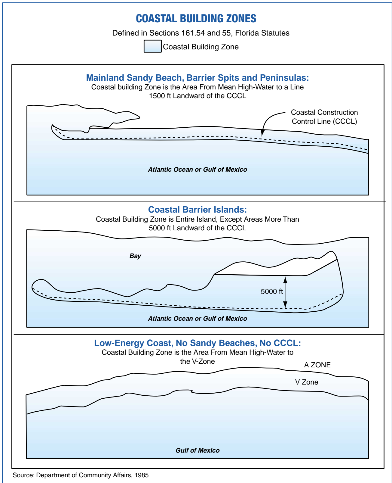
Figure G-6 Coastal construction building zones in Florida.
