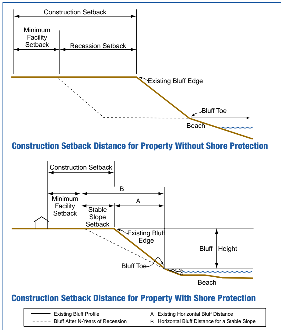
Figure G-17 Recommended coastal bluff setbacks (from Keillor 1998).
