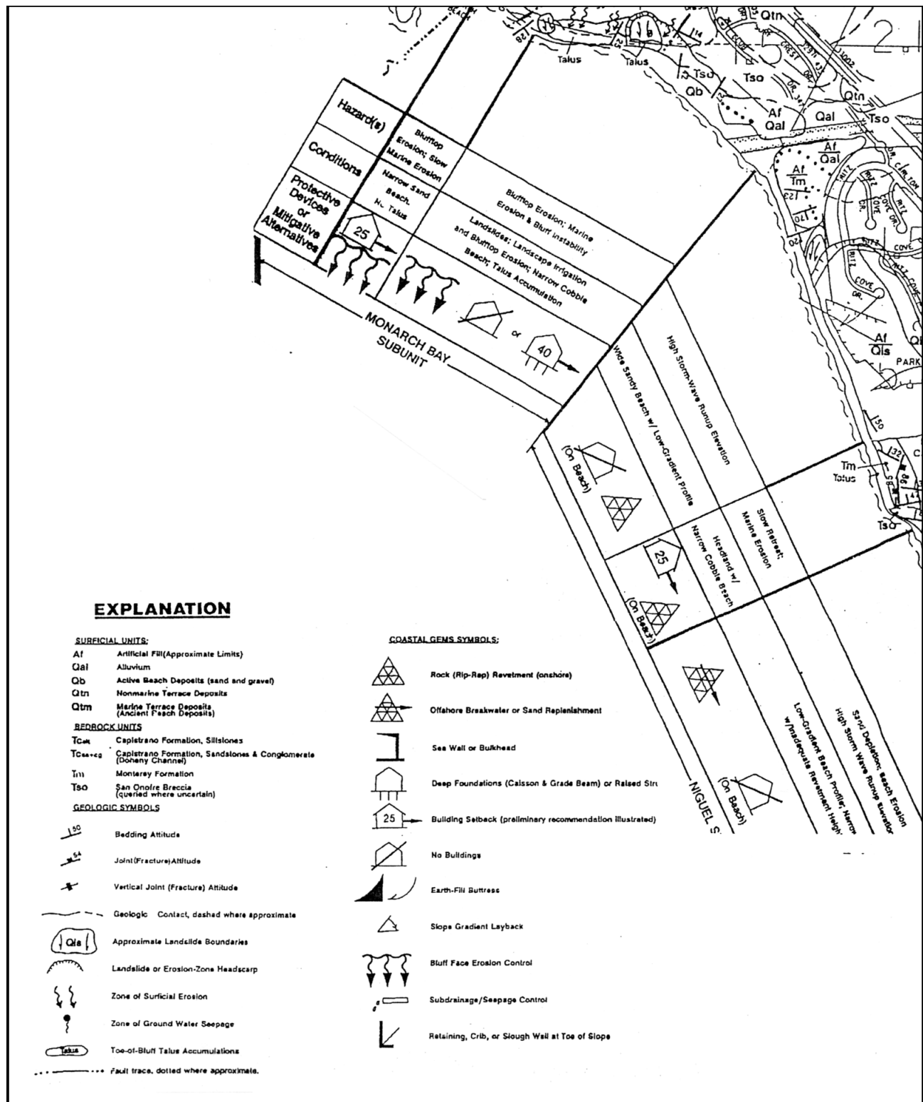
Figure G-15 Coastal erosion hazard and mitigation map, City of Dana Point, California (from Zeizer Geotechnical 1990).
