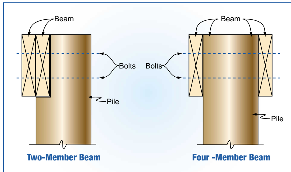
Figure 13-22 Proper pile notching for two- member and four-member beams.
